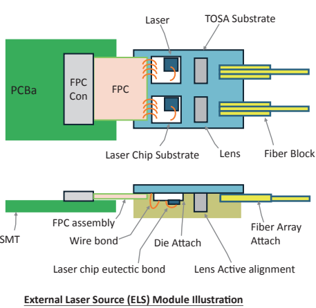
External Laser Source (ELS) Module Illustration
